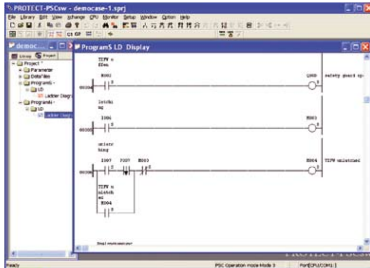
Fig. 6: Programming environment
